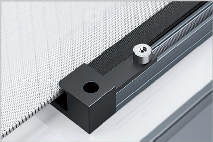
The new upgraded zipper guider allows the zipper to enter the plastic track smoothly and prevent the zipper from derailing.
