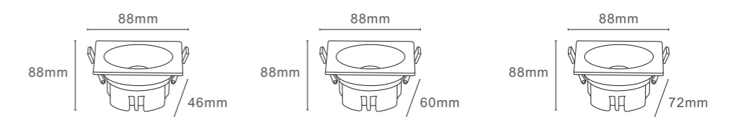
MODEL : CD-2332-7W/12W/15W Cutout:75mm
