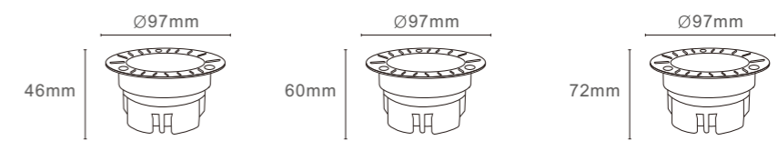
MODEL : CD-2332-7W/12W/15W Cutout:75mm
