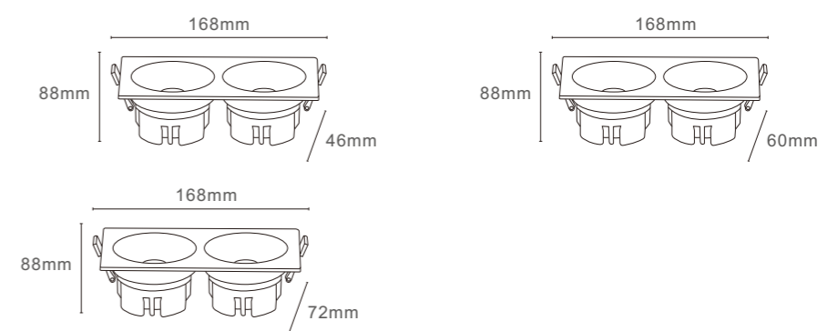
MODEL : CD-2332-2*7W/2*12W/ 2*15W Cutout:160*75mm
