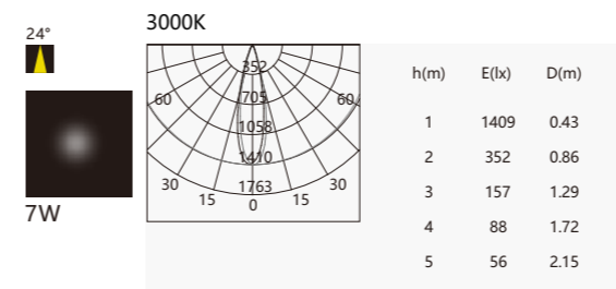
MODEL : CD-2332-7W/12W/15W Cutout:75mm
