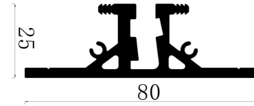
Components for Wall paneling and metal shelves
