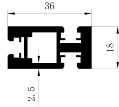
Aluminum back pole of middle side
