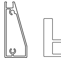
Alu frame for glass door and alu handle frame for glass door
