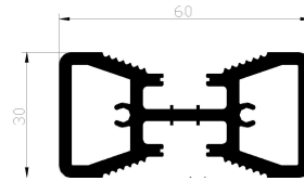
Aluminum pole
