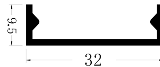
Edge banding of Wall paneling and metal shelves-B
