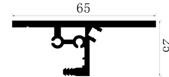
Upper and lower parts for Wall paneling and metal shelves
