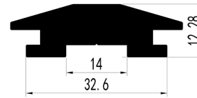
Shelf support
