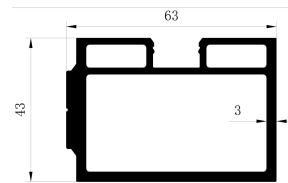
Profiles for aluminum base box
