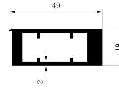
Profiles for fix air hinges
