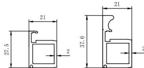
Alu frame for glass door and alu handle frame for glass door
