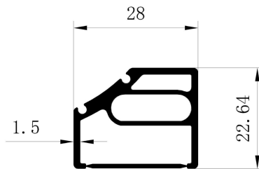
Aluminum profiles for wine bottle rack
