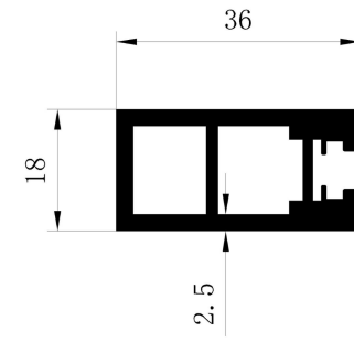
Front aluminum pole
