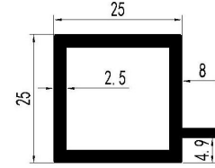
Profile with stop bar
