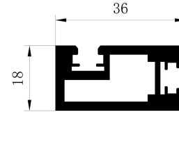
Back pole of side panel
