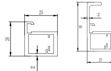
Alu frame for glass door and alu handle frame for glass door
