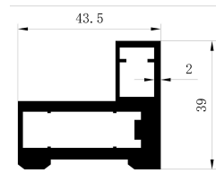
Front part for top and bottom frame
