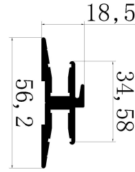
Rack buckle for L-shaped plate
