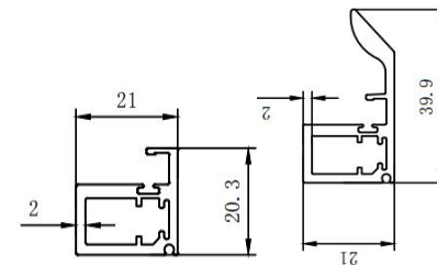
Alu frame for glass door and alu handle frame for glass door
