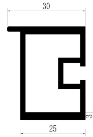
Back aluminum structure
