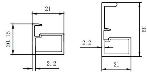
Alu frame for glass door and alu handle frame for glass door
