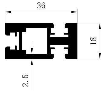
Aluminum back pole of middle side
