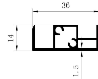
36mm profiles for glass shelf (Double glass)
