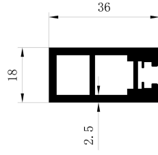
Front aluminum pole
