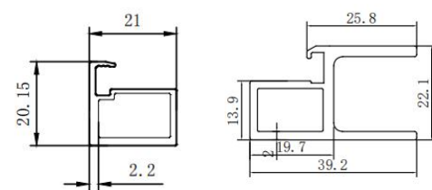
Alu frame for glass door and alu handle frame for glass door
