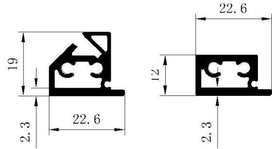
22 mm profiles for glass shelf (with silicone lamp cover)
