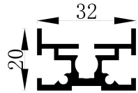
Support pole
