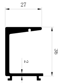
Aluminum profiles for Cup holder
