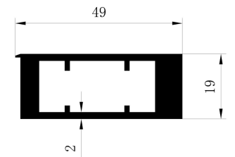
Profiles for fix air hinges
