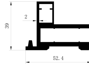
Left, right and back part for top and bottom frame
