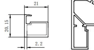
Alu frame for glass door and alu handle frame for glass door
