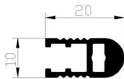
Aluminum profiles for glass shelf (Front part)
