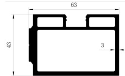
Profiles for aluminum base box
