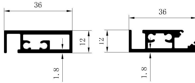
36mm profiles for glass shelf (with light trough)
