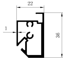
36mm profiles for glass shelf (Four sides with lights)
