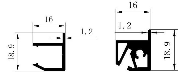
18 mm profiles for glass shelf (with silicone lamp cover)
