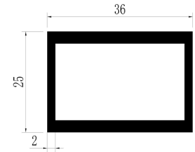
Beam for wood cabinets with aluminum structure
