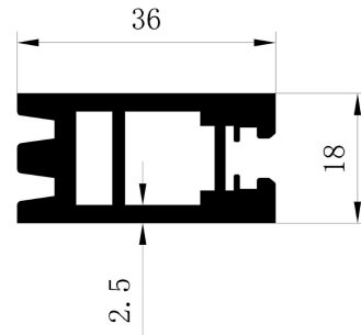
Front part for top and bottom panel of middle side
