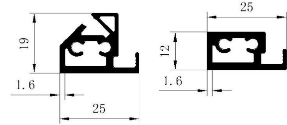
25 mm profiles for glass shelf (with silicone lamp cover)
