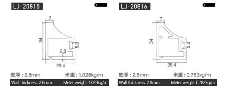
重型弧形天地框 Heavy-duty curved sky frame
