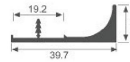
G-046G(Apple model)
