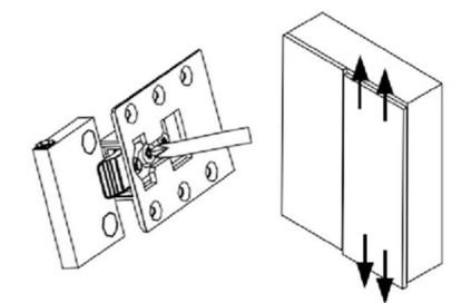
高度调节 Height adjustment: +/-2mm
