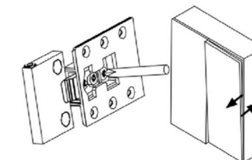
门板与侧板间隙调节: +/-1.5mm Adjustment of gap between door panel and side panel: +/-1.5mm
