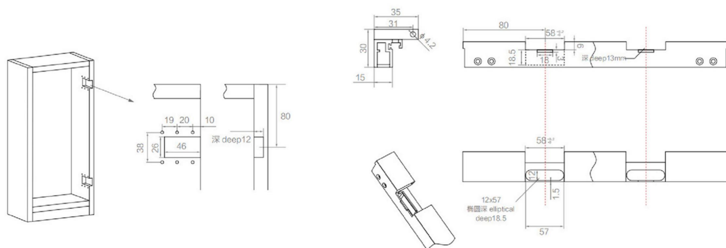
Hole size of cabinet side panel 柜体侧板开孔尺寸
