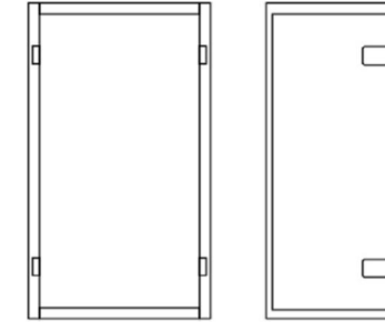
框体侧板开孔尺寸图 Size drawing of side plate of frame body
