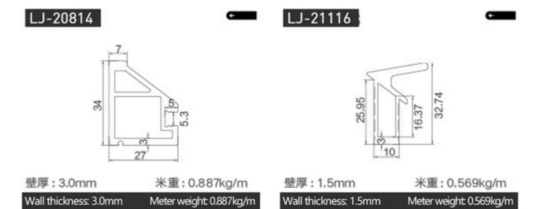
重型内嵌拉手天地框 Heavy built-in handle frame
