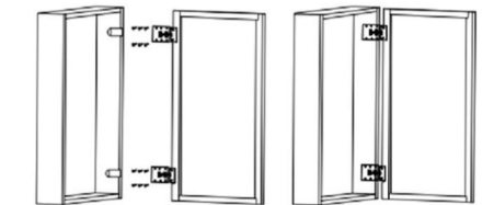
铝框门与柜体安装 Aluminum frame door and cabinet mounting
