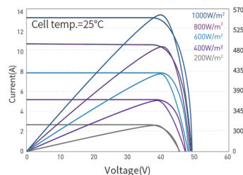
I-V curves/P-V curves of module under different irradiation(545w)
