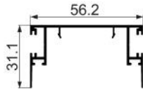
KY01-032 52 panels double vertical door frame with hook Weight : 0.5 kg/m
