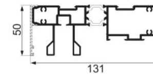
JNW-GD925F lifting top rails Weight : 2.75 kg/m
