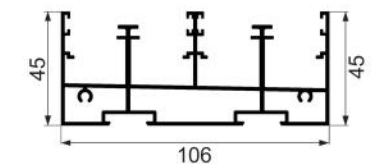
KY01-003F two-track high track Weight : 2.0 kg/m
