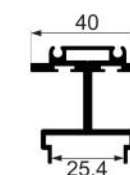
KY01-025 suspended track Weight : 0.94 kg/m
