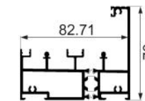
JNW-CT1676F two-track suspended bottom rail(landing) Weight : 2.29 kg/m
