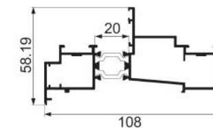
JNW-FK823A inward-opening subframe Weight : 1.59 kg/m
