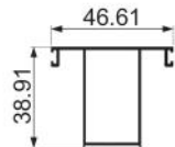
JNW-XT1331 side frame double cover Weight : 0.48 kg/m
