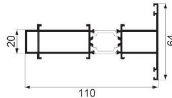
JNW-ZH813A injection molded center post Weight : 1.91 kg/m
