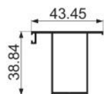
JNW-XT1332F side frame single cover Weight : 0.43 kg/m
