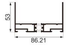
JNW-CT1416F two rail side seal Weight : 1.4 kg/m
