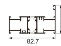
JNW-CT1343E two tracks fixed up and down Weight : 1.44 kg/m
