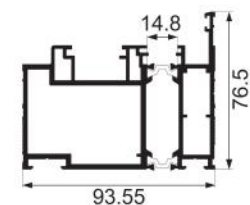
JNW-CT07-03 entrance door side sash Weight : 3.36 kg/m
