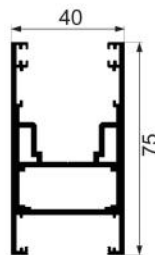
KY01-049 3.0-75 lifting panels Weight : 1.82 kg/m
