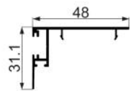
KY01-031 52 panels single vertical door frame with hook Weight : 0.32 kg/m
