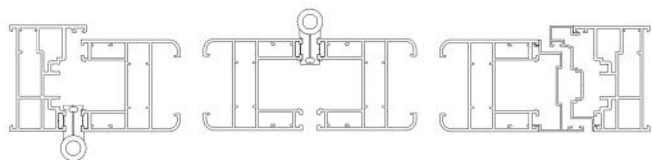
① 220 folding door assembly drawing:
