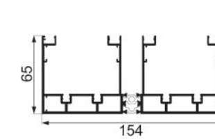
JNW-CT1805F2 pre-embedded double bottom tracks Weight : 3.7 kg/m
