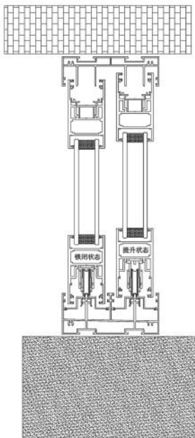
75 PROFILE DOUBLE TRACK ASSEMBLY DIAGRAM
