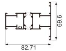
JNW-CT1343G two rail inner frame Weight : 1.61 kg/m
