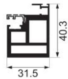
JNW-XT1466F mesh door with hook Weight : 1.22 kg/m
