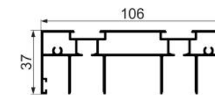
KY01-055 two-track Weight : 0.53 kg/m
