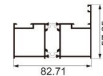
JNW-CT1420F two-track side frame transform Weight : 2.1 kg/m
