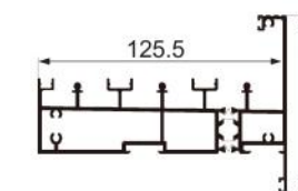
JNW-CT1460F three-track suspended bottom rail Weight : 3.22 kg/m
