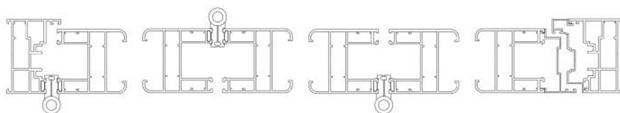
③ 330 folding door assembly drawing:
