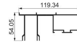
JNW-XT1186 intelligent top rail additional groove Weight : 1.86 kg/m
