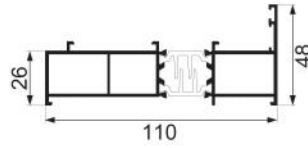
JNW-BK812A injection molded frame Weight : 1.77 kg/m
