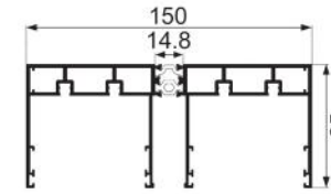
JNW-CT1798F2 double top tracks and side seals Weight : 3.44 kg/m
