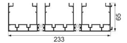
JNW-CT1805F3 three-track pre-embedded bottom tracks Weight : 5.61 kg/m
