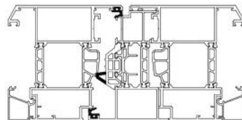
90 glass panel, double doors + outward-opening
