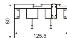
JNW-CT1485F three-track suspended upper rail Weight : 3.19 kg/m
