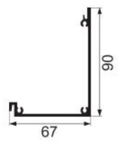
JNW-XT1890 additional drainage channels Weight : 1.16 kg/m
