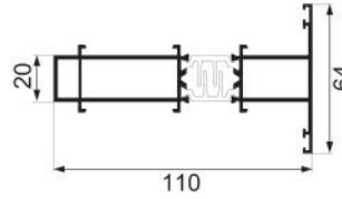
JNW-ZH813A injection molded center post Weight : 1.91 kg/m
