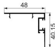
KY01-022 65 panels single vertical door frame with hook Weight : 0.35 kg/m
