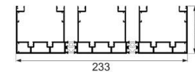
JNW-CT1813F3 panoramic door with three-track bottom tracks Weight : 5.54 kg/m
