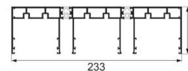
JNW-CT1811F3 three-track top tracks and side seals Weight : 5.25 kg/m
