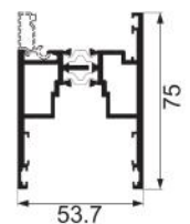
JNW-TS1917F inside slim vertical door frame Weight : 2.1 kg/m
