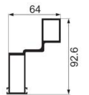
JNW-XT1863 intelligent track with additional material in the middle Weight : 1.62 kg/m
