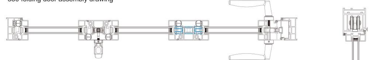
321 folding door assembly drawing
