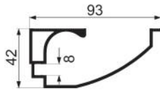
XY03-012 light strip handle Weight : 1.33 kg/m
