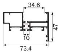
DZ-CT795F slim glass sash Weight : 1.42 kg/m
