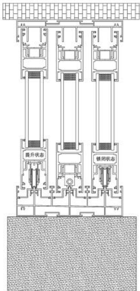
75 PROFILE TRIPLE TRACK ASSEMBLY DIAGRAM
