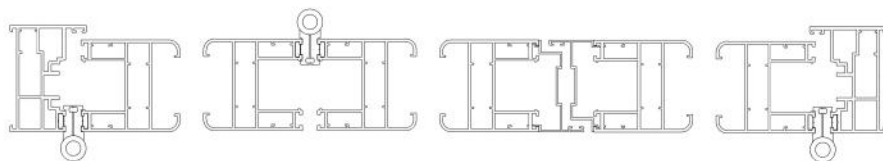
② 321 folding door assembly drawing:
