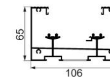
KY01-009 two-track suspended track Weight : 2.33 kg/m
