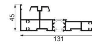
JNW-GD919F lifting bottom rail Weight : 2.6 kg/m
