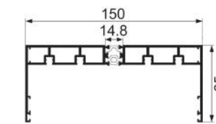
JNW-CT1861F intelligent double top tracks Weight : 2.9 kg/m
