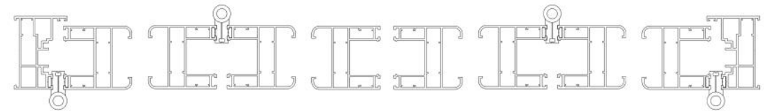
⑤ 431 folding door assembly drawing:
