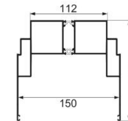
JNW-CT1862F intelligent additional top track Weight : 4.5 kg/m
