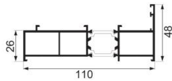
JNW-BK812A injection molded frame Weight : 1.77 kg/m
