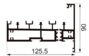
JNW-CT1708F 3.0 three-track suspended bottom rail Weight : 4.06 kg/m
