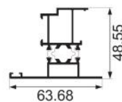
HC235B center frame for glass fans Weight : 1.05 kg/m
