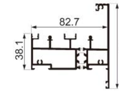
JNW-CT1459F two-track suspended bottom rail Weight : 2.4 kg/m
