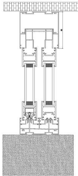
52 PROFILE ELECTRIC ASSEMBLY DIAGRAM
