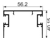
KY01-023 65 panels double vertical door frame with hook Weight : 0.56 kg/m
