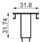
JNW-XT1468 bottom double side frame cover Weight : 0.39 kg/m
