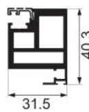
JNW-XT1671 outside mesh door with hook Weight : 1.3 kg/m
