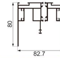
JNW-CT1487F two-track suspended upper rail Weight : 2.4 kg/m
