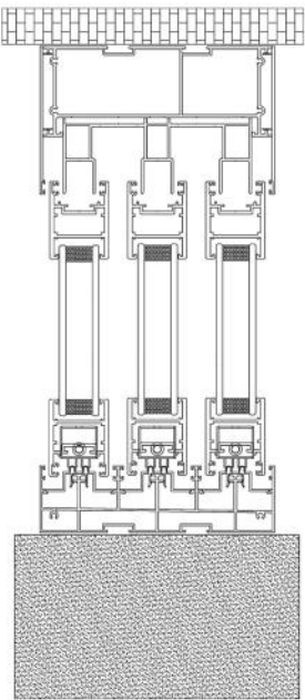
75 PROFILE ELECTRIC ASSEMBLY DIAGRAM
