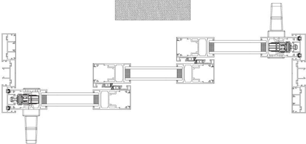
75 PROFILE ELECTRIC ASSEMBLY DIAGRAM
