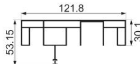
JNW-XT1586 suspended window intelligent upper track additional track Weight : 1.99 kg/m
