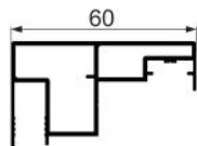
JNW-A-042 60 wall cover frame Weight : 0.8 kg/m
