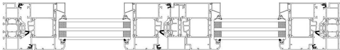
90 glass panel, double doors + inward-opening
