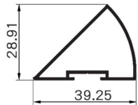
SK661 Name : lock profile for 1+ 1 Thickness : 1.0mm Weight : 0.33 kg/m
