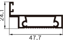
D-A630 Name : closing Thickness : 1.2mm Weight : 0.63 kg/m
