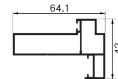
D-A563H Name : push in door Jamb Thickness : 1.2mm Weight : 0.84 kg/m
