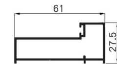
D-A566 Name : push in door Jamb Thickness : 1.2mm Weight : 0.63 kg/m
