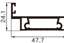
D-A630 Name : closing Thickness : 1.2mm Weight : 0.63 kg/m
