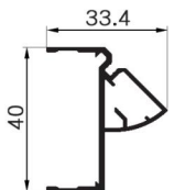
OPK-A206 Name : 45 degrees corner Thickness : 1.5mm Weight : 0.42 kg/m
