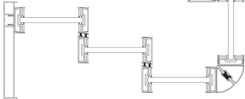
40 system universal corner
