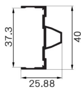
OPK-A207 Name : collision cover Thickness : 1.5mm Weight : 0.36 kg/m
