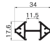
D145 Name : glass divider Thickness : 1.5mm Weight : 0.44 kg/m
