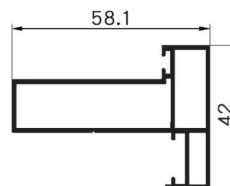
D-A613 Name : semi-recessed door frame Thickness : 1.2mm Weight : 0.79 kg/m
