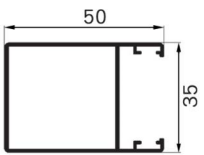
SK780 Name : door frame Thickness : 1.2mm Weight : 0.62 kg/m
