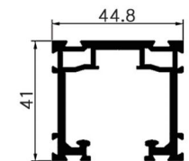
OPK-A101H Name : hanging rail Thickness : 2.5mm Weight : 1.35 kg/m
