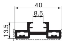
SK733A Name : vertical door frame Thickness : 1.5mm Weight : 0.49 kg/m
