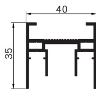
SK728 Name : top and bottom frame Thickness : 1.5mm Weight : 0.72 kg/m
