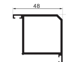
WB-80007 Name : double glass corner column Weight : 0.903 kg/m
