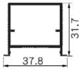
D-A580 Name : support pole (4/5mm) Thickness : 1.4mm Weight : 0.53 kg/m
