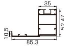
JY-WP-96 Name : door frame (interior lock) Weight : 1.28 kg/m
