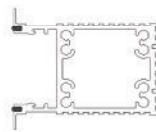
▼ 1.8*3.3 rubber for door panel vertical frame (0276)
