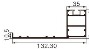
JY-WP-82 Name : door frame (interior lock) Weight : 1.57 kg/m
