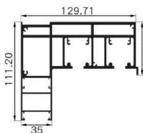
JY-35PT-06 Name : three door top horizontal outframe Weight : 6.09 kg/m
