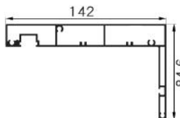
JY-WP-14 Name : three door top horizontal outframe Weight : 2.07 kg/m
