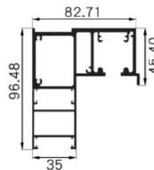
JY-35PT-02 Name : two door top horizontal outframe Weight : 3.28 kg/m
