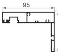
JY-WP-02 Name : two door top horizontal outframe Weight : 1.55 kg/m
