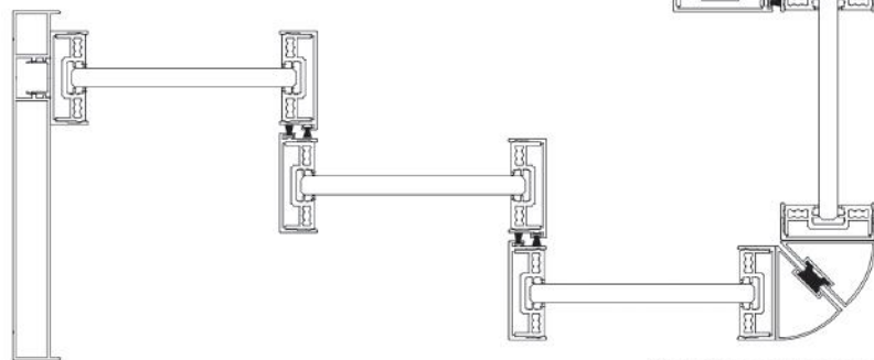
40 system universal corner
