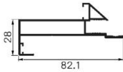
D-A571 Name : main frame Thickness : 1.4mm Weight : 0.94 kg/m
