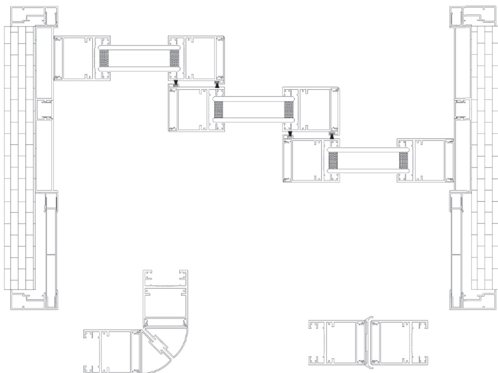
40 system universal corner
