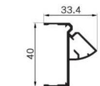
OPK-A206 Name : 45 degrees corner Thickness : 1.5mm Weight : 0.42 kg/m
