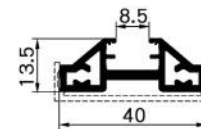
SK734A Name : vertical door frame Thickness : 1.5mm Weight : 0.51 kg/m
