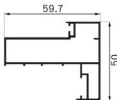
D-A614 Name : front wall cover Thickness : 1.1mm Weight : 0.8 kg/m
