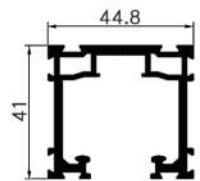
OPK-A101H Name : hanging rail Thickness : 2.5mm Weight : 1.35 kg/m
