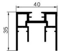
SK731A Name : top and bottom frame Thickness : 1.5mm Weight : 0.78 kg/m
