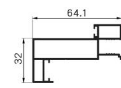
D-A562 Name : push in door Jamb Thickness : 1.2mm Weight : 0.88 kg/m
