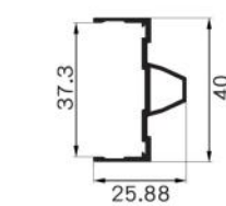
OPK-A207 Name : collision cover Thickness : 1.5mm Weight : 0.36 kg/m
