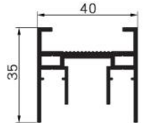
SK728 Name : top and bottom frame Thickness : 1.5mm Weight : 0.72 kg/m
