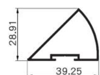
SK661 Name : lock profile for 1+ 1 Thickness : 1.0mm Weight : 0.33 kg/m
