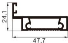
D-A630 Name : closing Thickness : 1.2mm Weight : 0.63 kg/m
