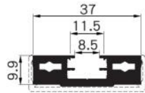
SK790 Name : vertical door frame Thickness : 5.0mm Weight : 0.69 kg/m
