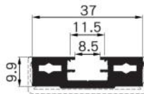
SK790 Name : vertical door frame Thickness : 5.0mm Weight : 0.69 kg/m
