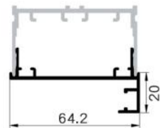
(equal width folding) C379 Name : vertical outer frame Weight : 0.55 kg/m
