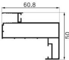
D-A615 Name : reverse wall cover Thickness : 1.1mm Weight : 0.82 kg/m
