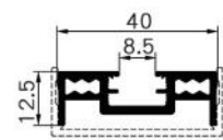
SK732A Name : vertical door frame Thickness : 1.5mm Weight : 0.48 kg/m
