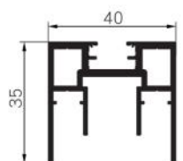
SK731A Name : top and bottom frame Thickness : 1.5mm Weight : 0.78 kg/m
