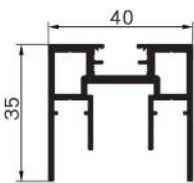
SK731A Name : top and bottom frame Thickness : 1.5mm Weight : 0.78 kg/m
