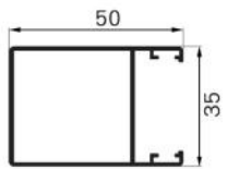
SK780 Name : door frame Thickness : 1.2mm Weight : 0.62 kg/m
