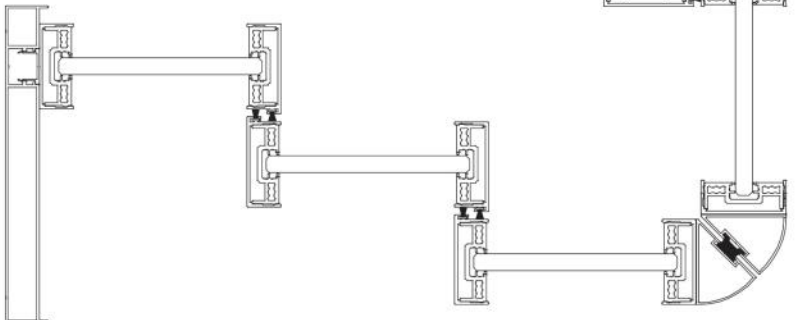
40 system universal corner
