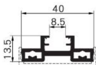
(for install top locks) SK817 Name : vertical door frame Thickness : 1.5mm Weight : 0.51 kg/m
