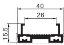
SK727 Name : vertical door frame Thickness : 1.5mm Weight : 0.51 kg/m
