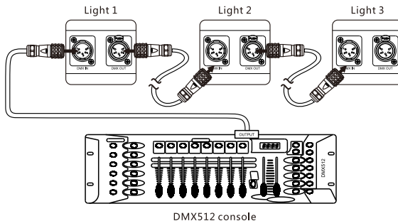
DMX connection for multiple lights
